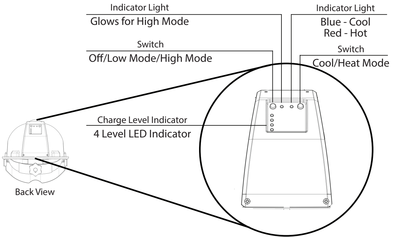
Fig. B - Control Panel - Kepi 2.0
